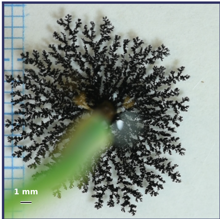
0.04 % D = 1.91
